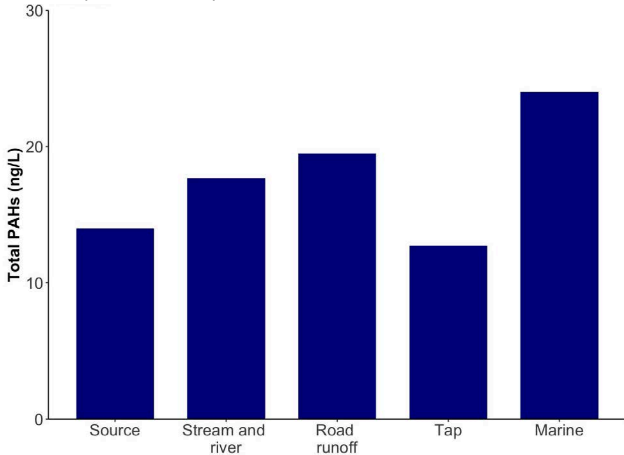
Figure 6: Total PAH concentrations in water samples from the Anderson Creek watershed (WET Season 2024)
