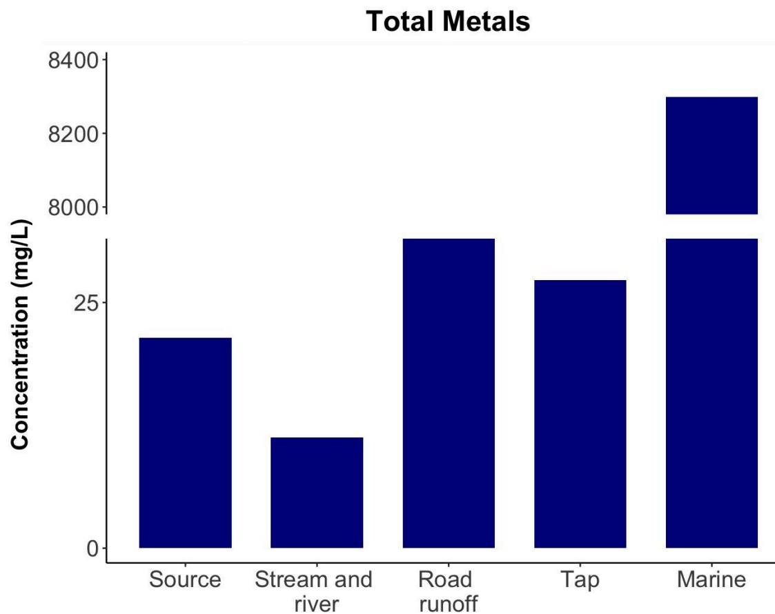
Figure 4: Total metal concentrations (mg/L) in water samples from the Anderson Creek watershed (WET Season 2024)
