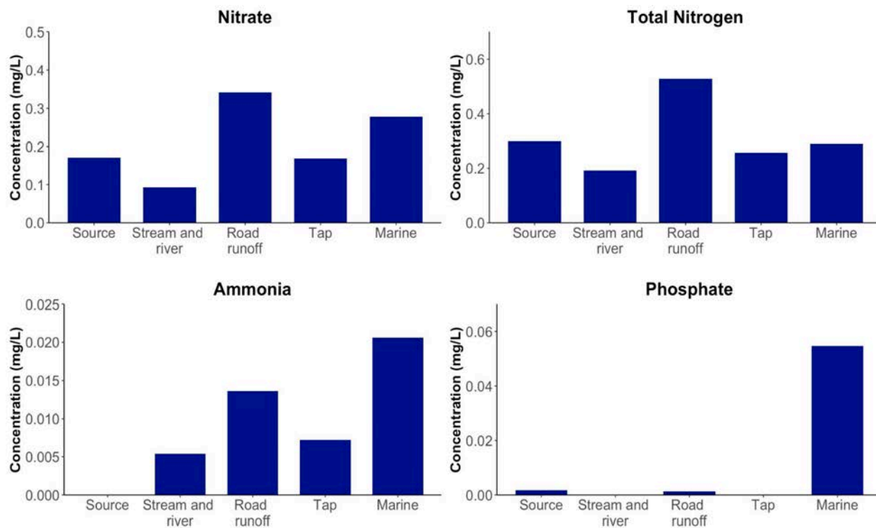
Figure 3: Mean Nutrient concentrations (mg/L) in water samples from the Anderson Creek watershed (WET Season 2024)
