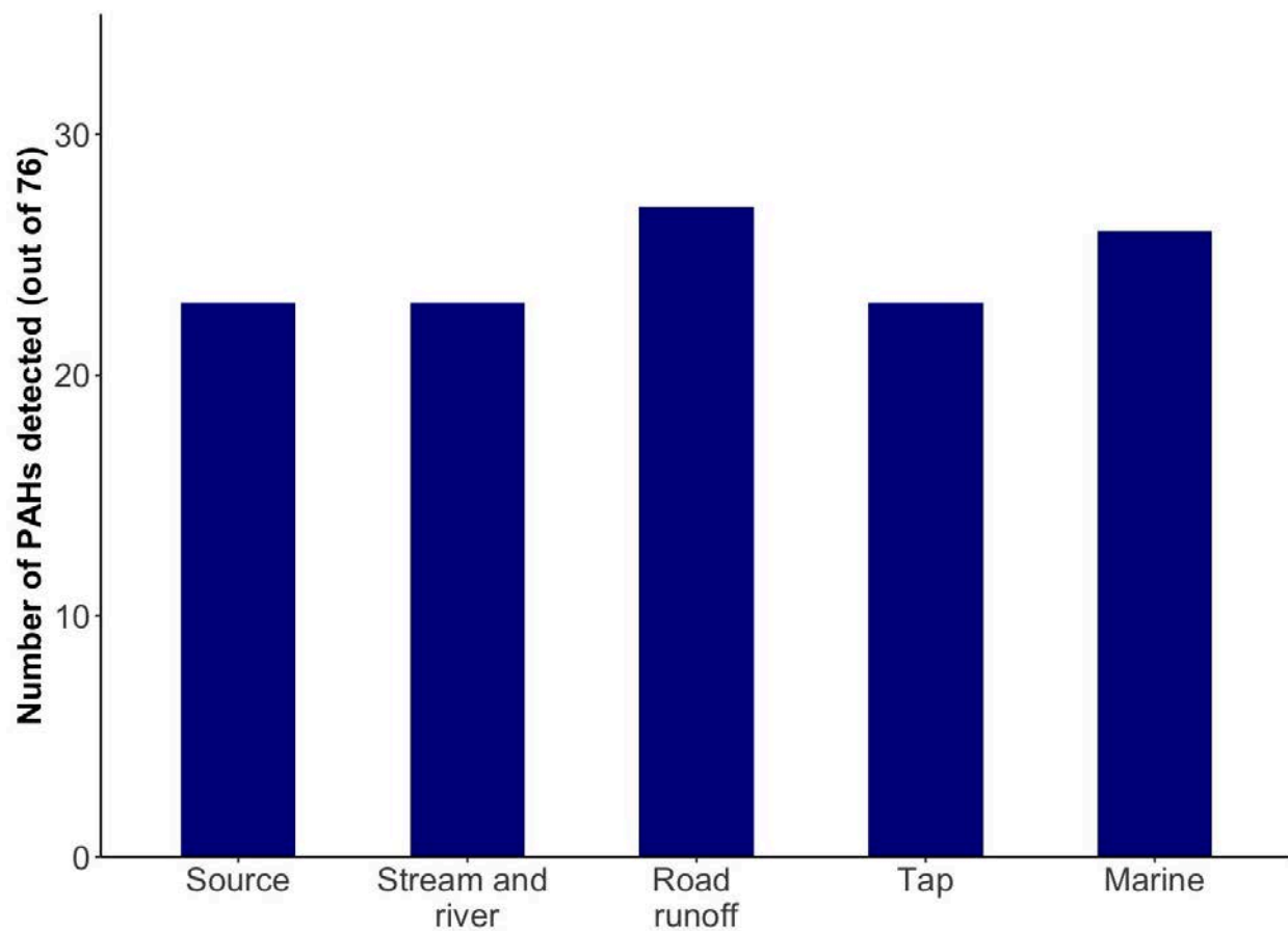
Figure 5: Number of PAHs detected in water samples from the Anderson Creek watershed (WET Season 2024)
