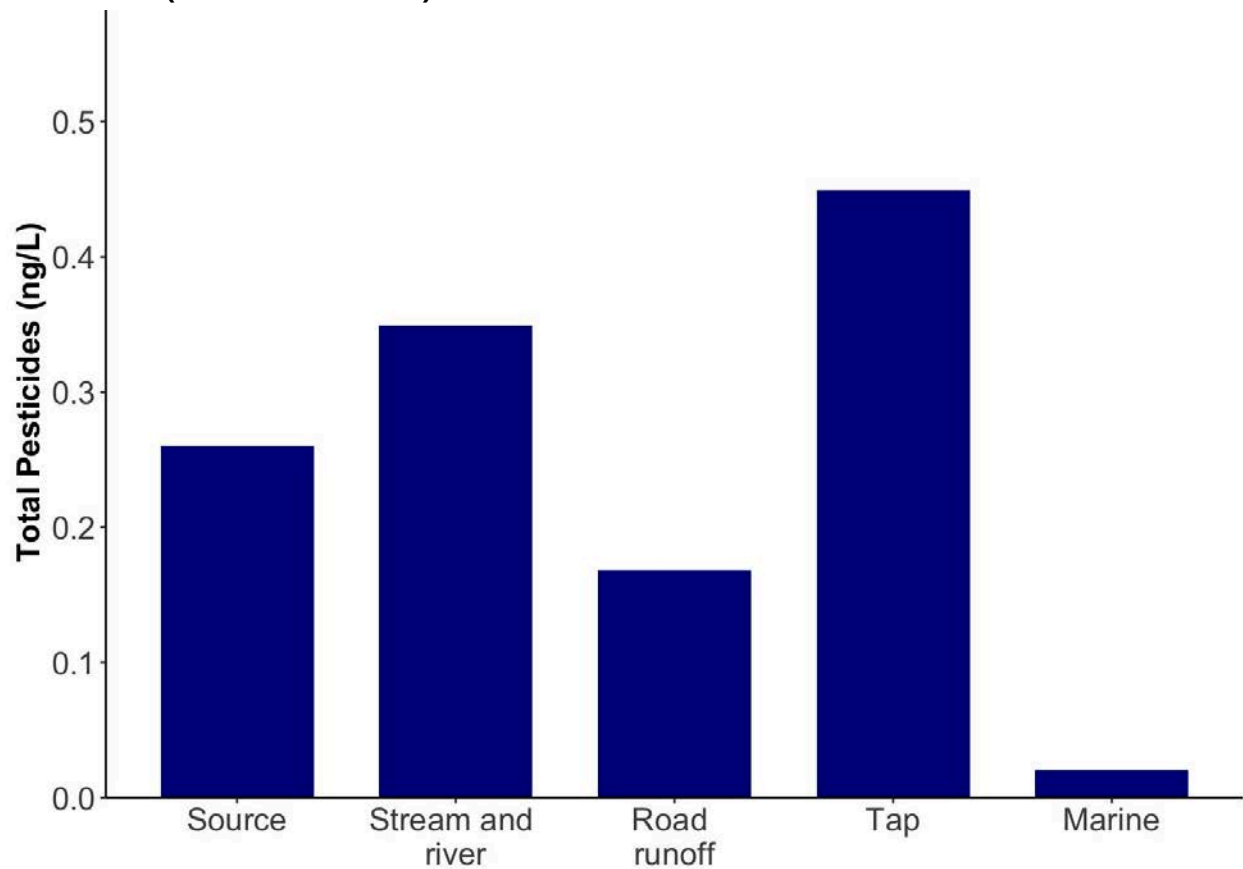
Figure 9: Total pesticide concentrations in water sampled in the Anderson Creek watershed (WET Season 2024)
