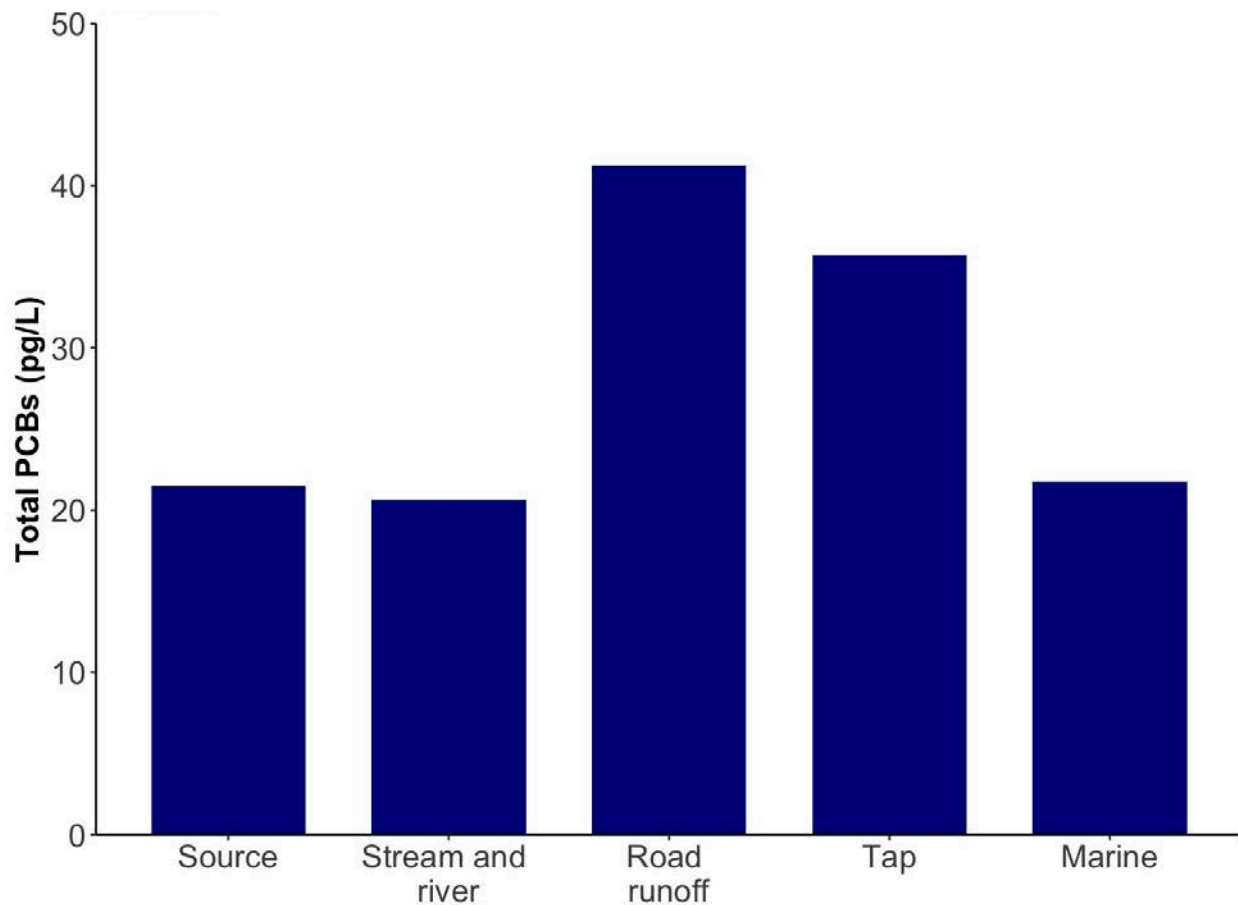
Figure 15: Total PCB concentrations in water sampled from the Anderson Creek watershed (WET Season 2024)
