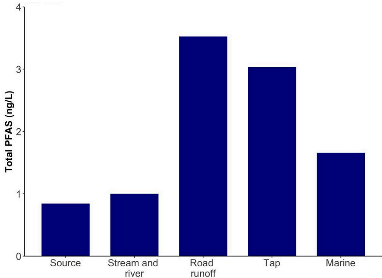
Figure 13: Total PFAS concentrations in water sampled in the Anderson Creek watershed (WET Season 2024)
