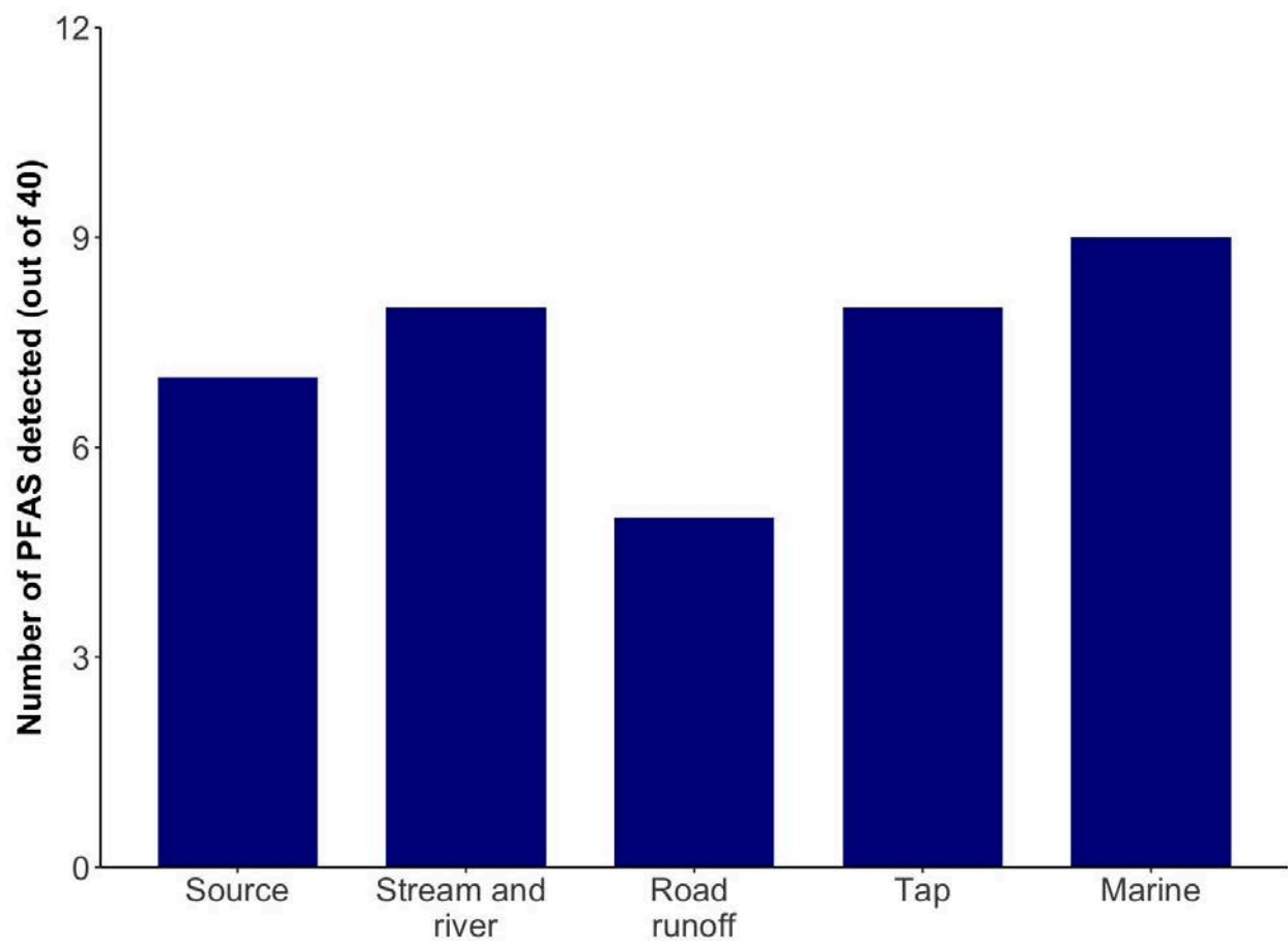
Figure 12: Number of PFAS substances detected in water samples from the Anderson Creek watershed (WET Season 2024)
