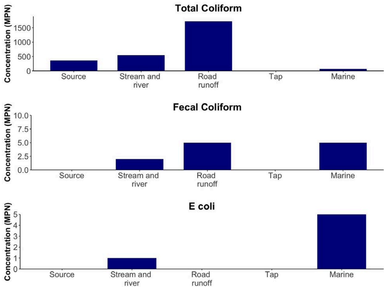
Figure 2: Coliform counts (MPN) in water samples from the Anderson Creek watershed (WET Season 2024)
