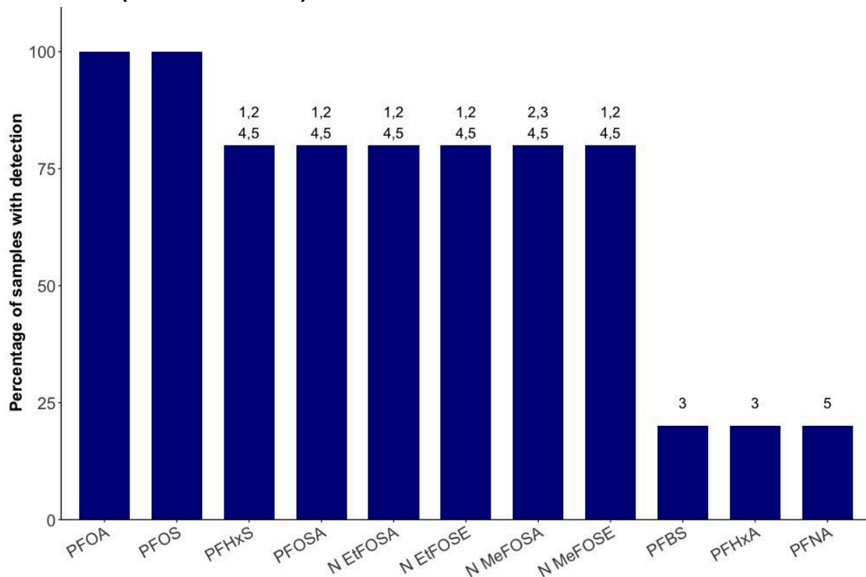
Figure 13: Most frequently detected PFAS in water sampled in the Anderson Creek watershed (WET Season 2024)
