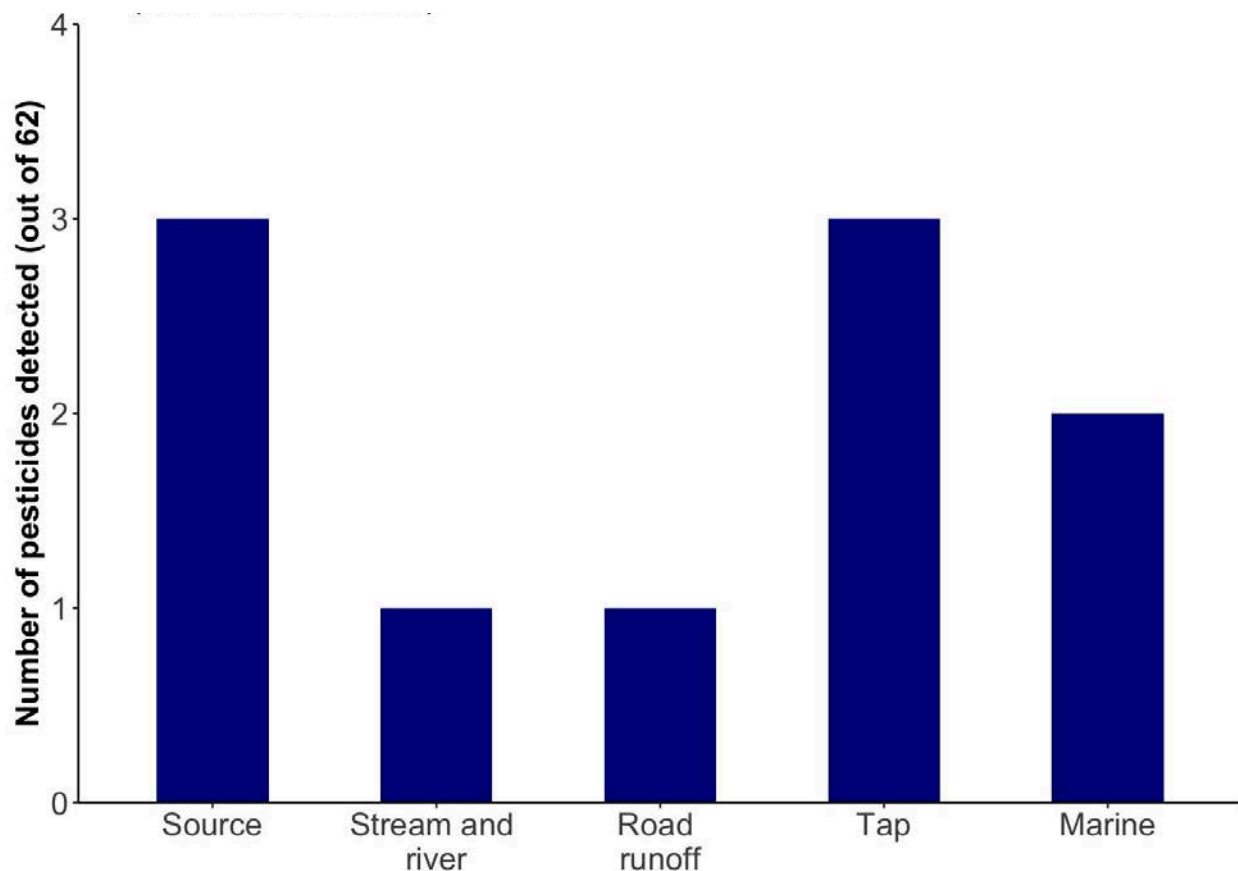
Figure 8: Number of pesticide detections in water sampled in the Anderson Creek watershed (WET Season 2024)
