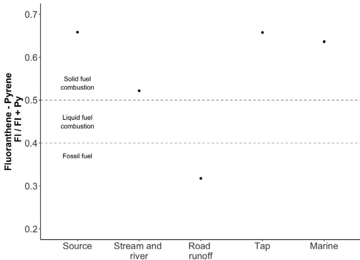
Figure 7: Hydrocarbon profiles from wood combustion and fuels in water samples from the Anderson Creek watershed (WET Season 2024)
