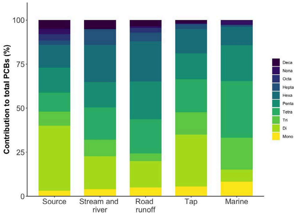
Figure 16: Homologue group contribution to total PCBs in water sampled from the Anderson Creek watershed (WET Season 2024)
