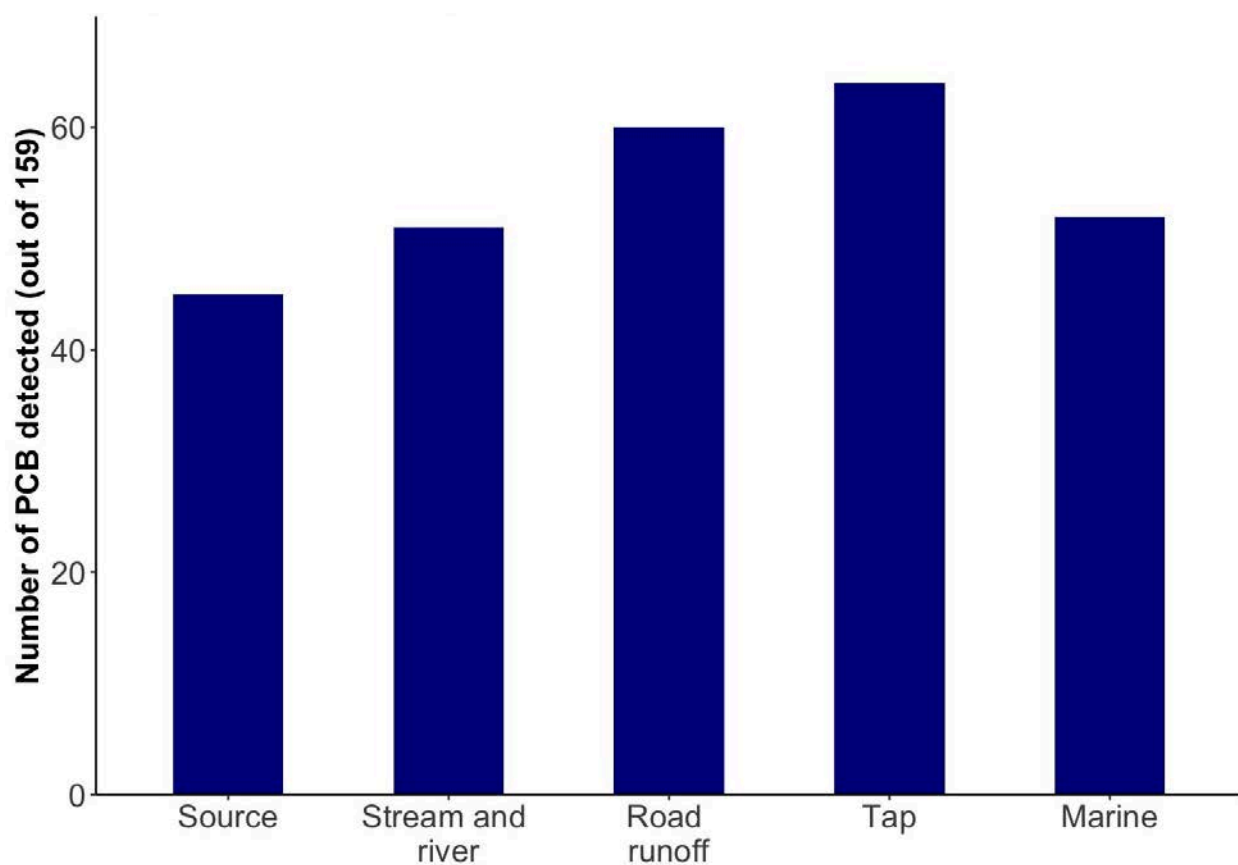
Figure 14: Number of PCB detections in water sampled from the Anderson Creek watershed (WET Season 2024)
